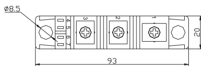
Fig. 8 - Outline Characteristics
