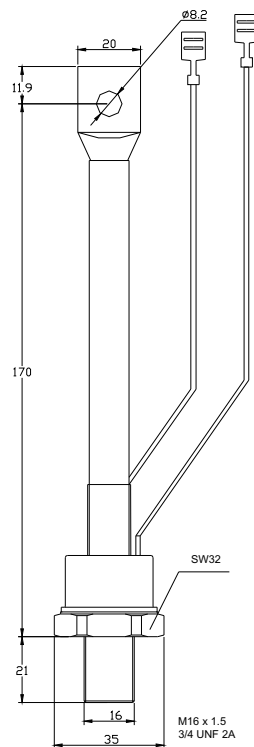
Fig. 8 - Outline Characteristics
